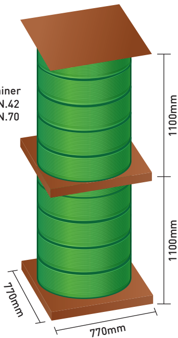
Pallet with 24+24 Coil
