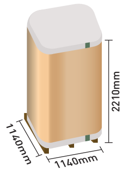
Pallet with 52 Coil
